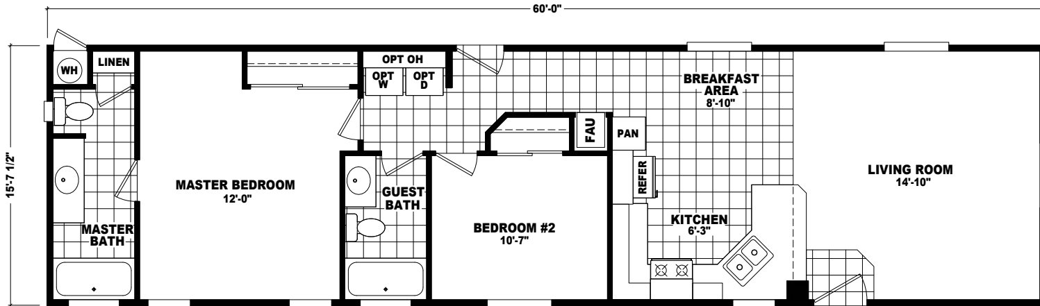
MODEL: EP-16602A APPROXIMATELY 937 SQ. FT. 2 BEDROOM, 2 BATH
