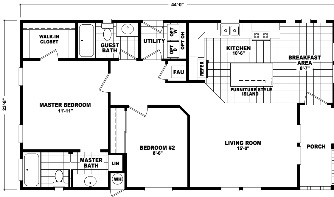
MODEL: WP-2442A APPROXIMATELY 1041 SQ. FT. TOTAL APPROXIMATELY 982 SQ. FT. LIVABLE 2 BEDROOM, 2 BATH
