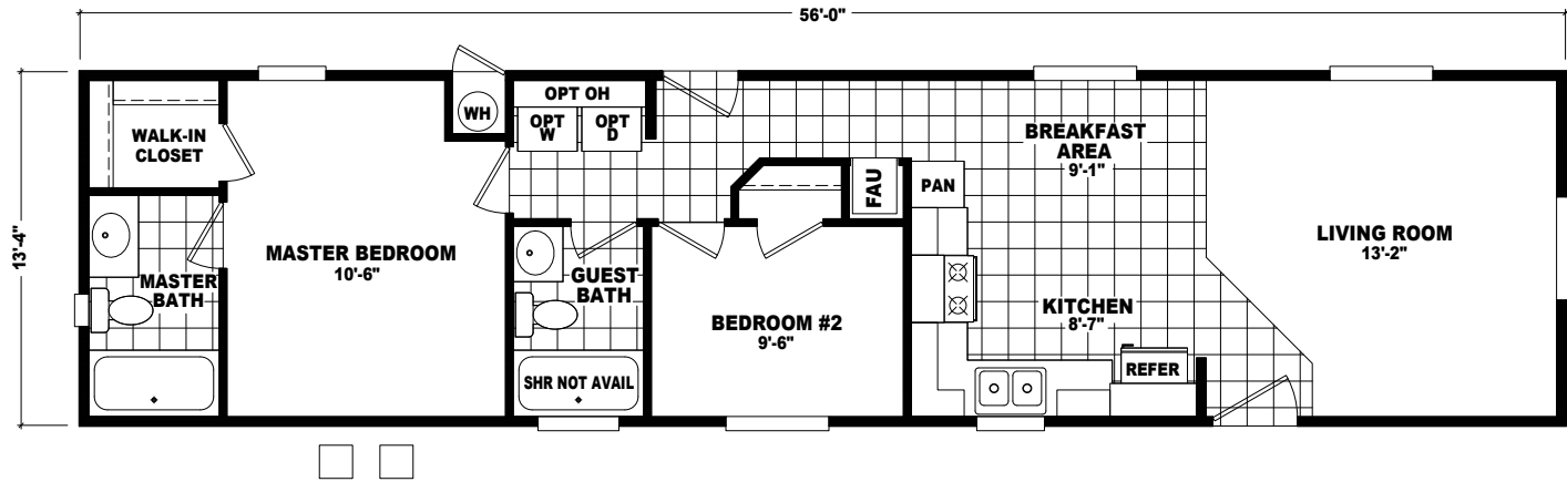
MODEL: EP-14562A APPROXIMATELY 746 SQ. FT. 2 BEDROOM, 2 BATH
