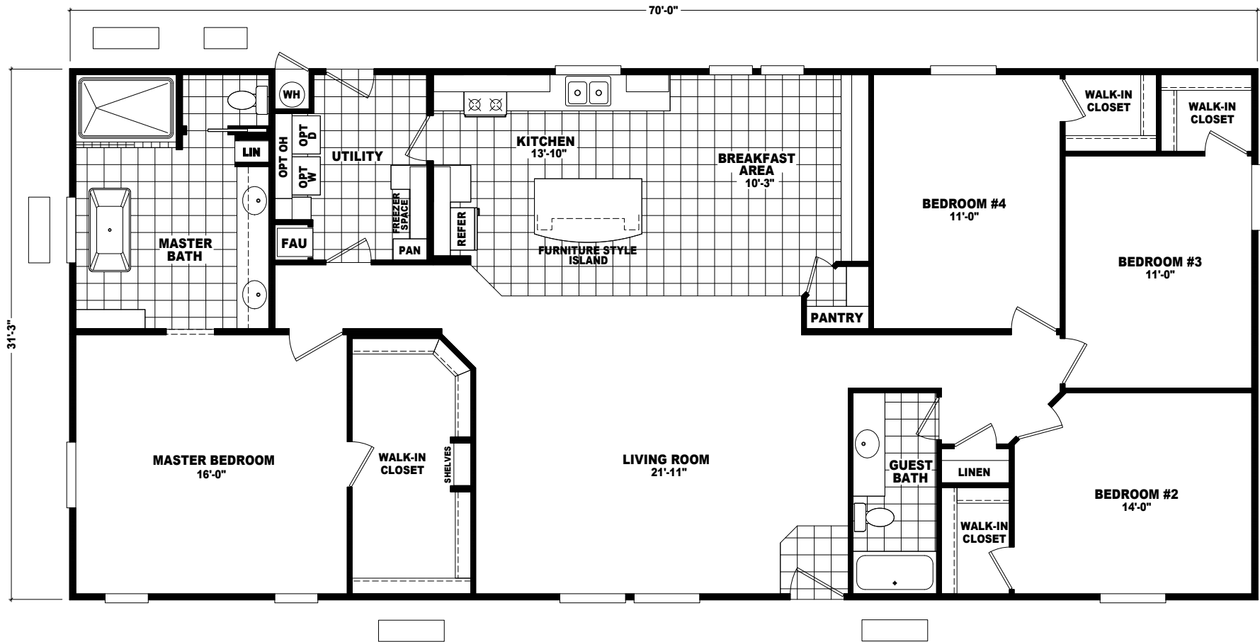
MODEL: DR-32704A APPROXIMATELY 2187 SQ. FT. 4 BEDROOM, 2 BATH
